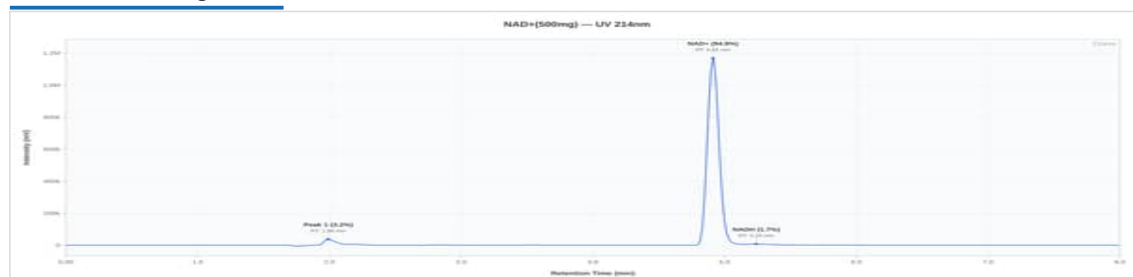
NAD+ 500mg - LU-NAD52.28.2026: UV Chromatogram
